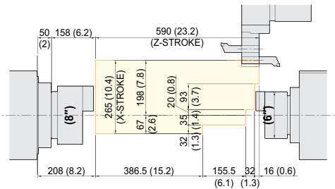
Angular driven Tool holder
