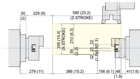
Axial driven Tool holder
