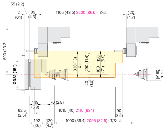
Angular driven
