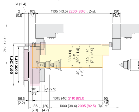
Angular driven
