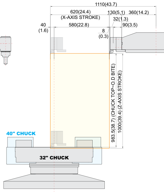
(FACING HOLDER)
