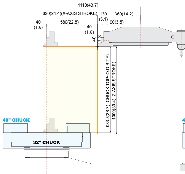
(O.D. HOLDER)
